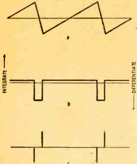
Fig. 3—Differentiation of a sawtooth wave.
