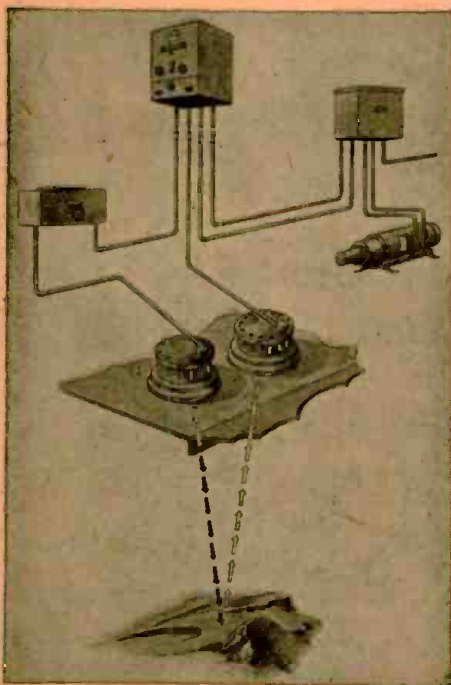
Fig. 3—Equipment of standard echo sounder.
