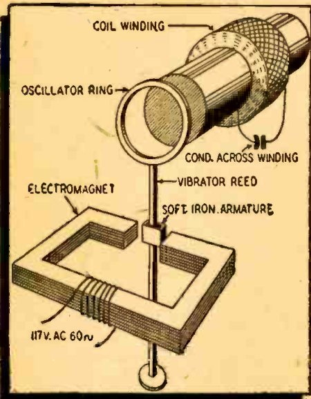
Fig. 1—Components of frequency wobbler.
