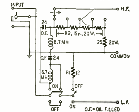
Fig. 5—A simple cross-over network.
