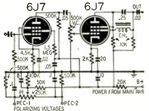
Fig. 3—Voltage amplifier for two soundheads.
