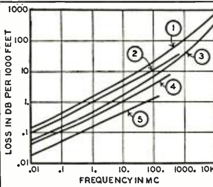
Fig. 7—Characteristics of co-axial cables.
