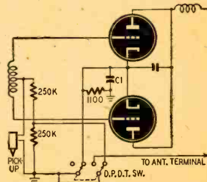
Fig. 5—Attachment to another special circuit.
