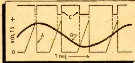
Diagram to illustrate pulse-width modulation.
