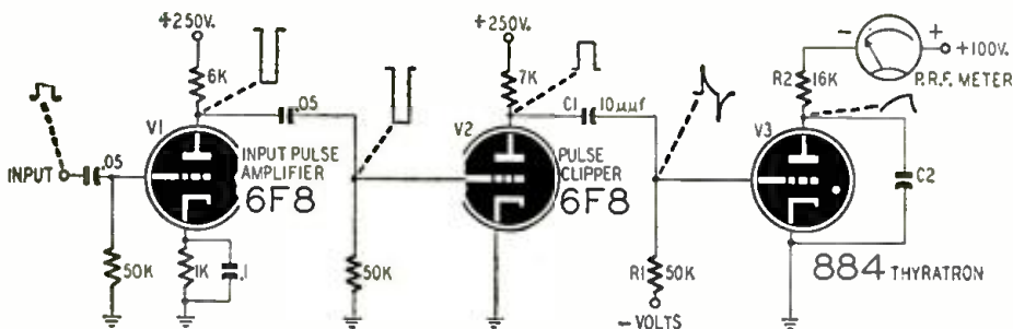
Fig. 3—Circuit of the pulse repetition frequency counter. Thyatron detail shown below.
