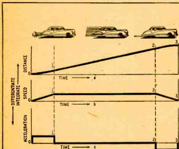
Fig. 1—Distance, speed and acceleration reproduced in graph form.
