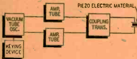
Fig. 1—One way of exciting transducer.
