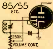
Fig. 4-a—Diode-biased detector-audio stage. Lack of bias on phonograph poses a problem.
