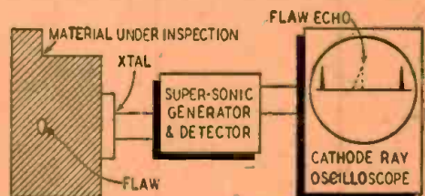
Fig. 4—Supersonic casting inspection hookup.
