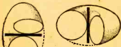
Fig. 1—Shape of the field around a dipole. Antenna is vastly exaggerated to be visible in the sketch.
