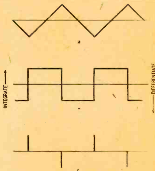
Fig. 2—Differentiation and integration in actual radio circuits.
