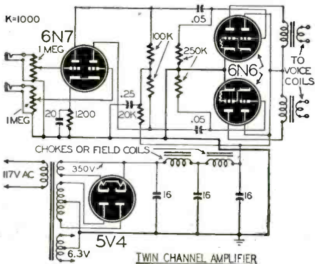
TWIN CHANNEL AMPLIFIER
