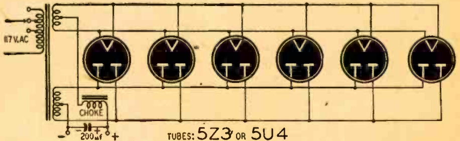
Fig. 2—A large bank of rectifiers excites the fields of several loudspeakers in parallel.
